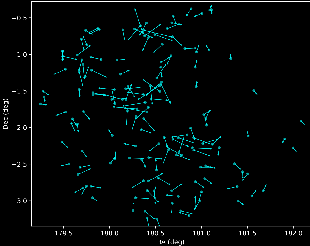
APOGEE DR17 Noise Stream Proper Motion Vectors (n=150)
