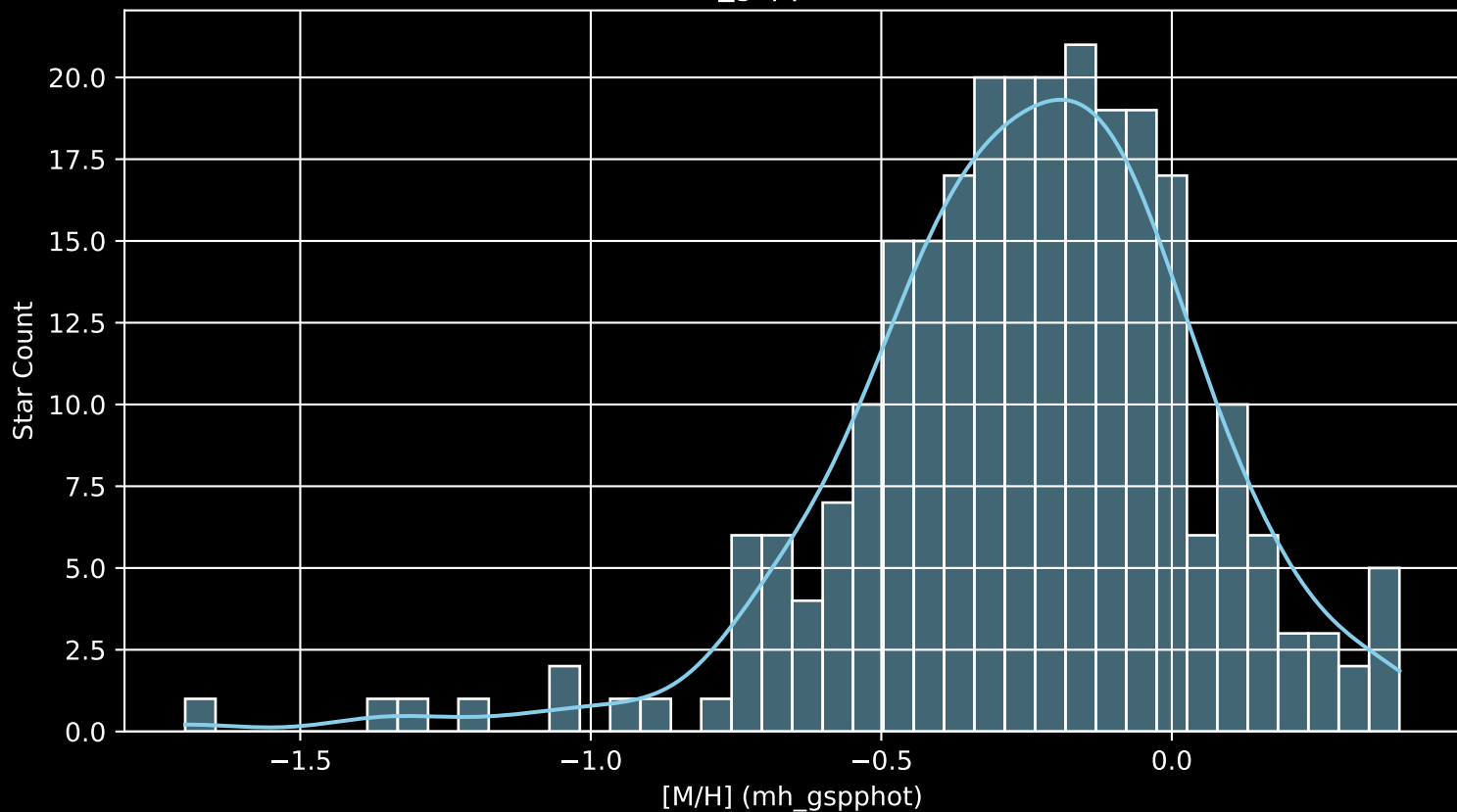
APOGEE DR17 Field: [ORIONOB1AB-D [M/H] (mh_gspphot) (n= 260)
