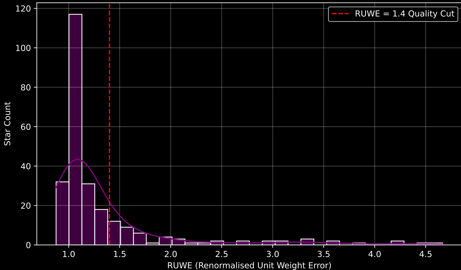
GAPOGEE DR17 Field [ORIONOB1AB-D] RUWE Distribution (n= 253)
