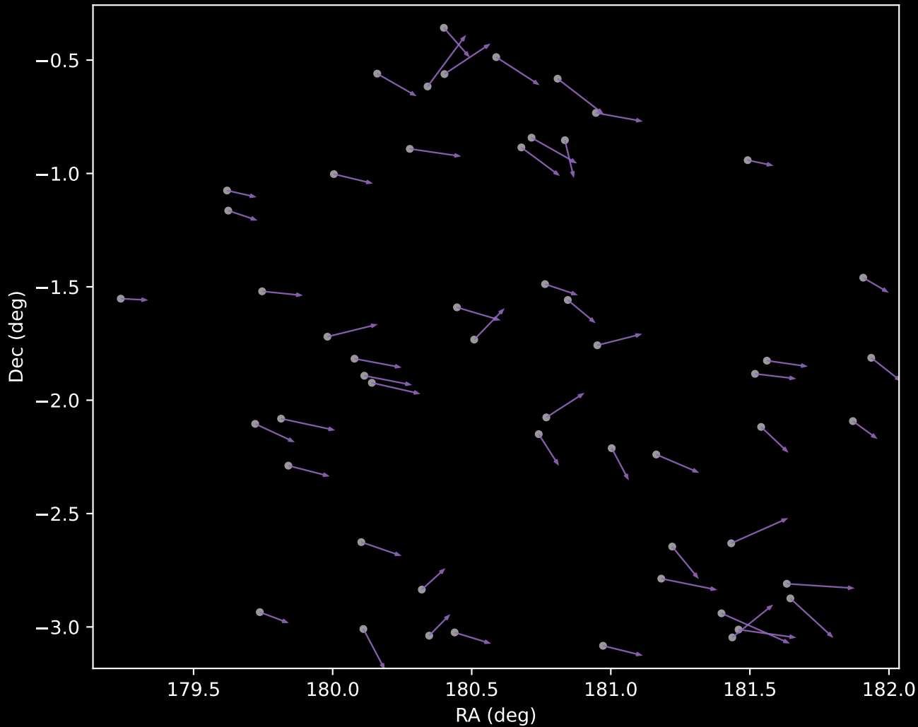
APOGEE DR17 Cluster 8 Proper Motion Vectors (n=54)
