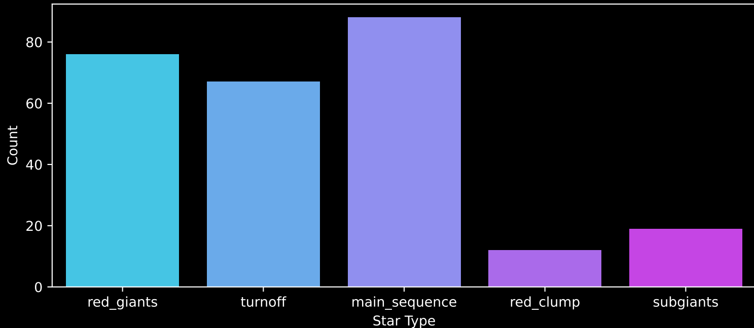
APOGEE DR17 Field: [ORIONOB1AB-D] Count plot of Star Type
