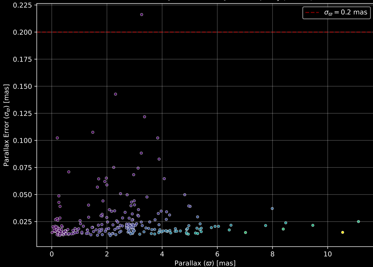
APOGEE DR17 Field: [ORIONOB1AB-D] Parallax Quality (n= 262)
