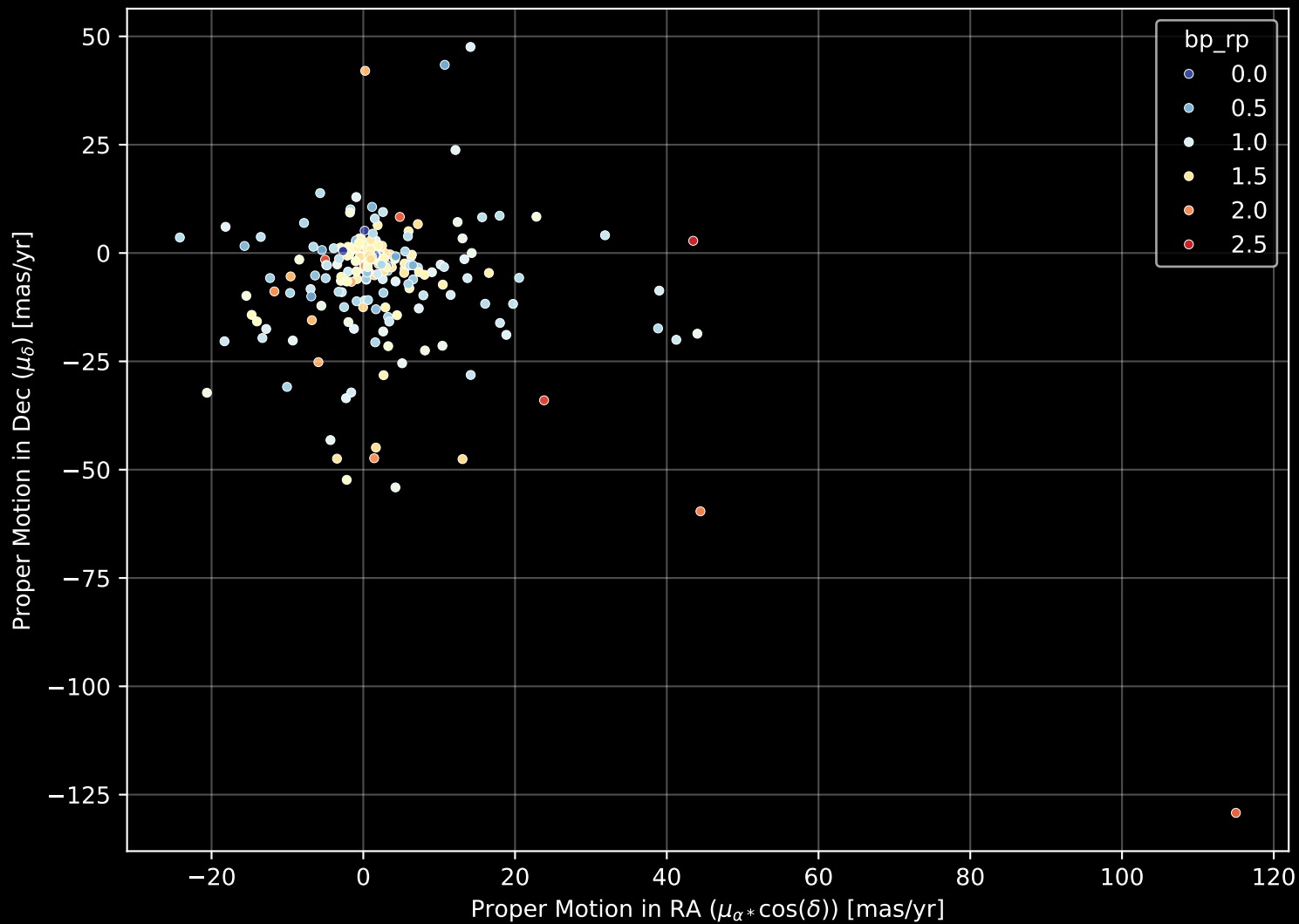
APOGEE DR17 Field: [ORIONOB1AB-D] Proper Motion Diagram (n= 262)
