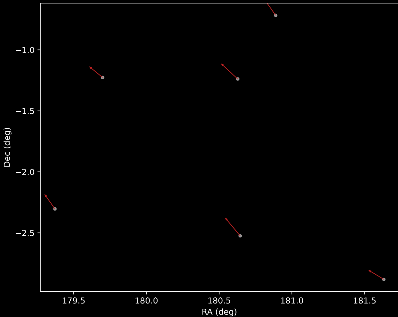
APOGEE DR17 Cluster 6 Proper Motion Vectors (n=6)
